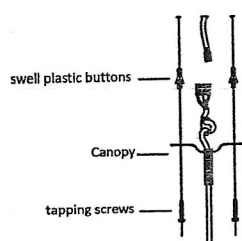
K. Install the swell plastic buttons into the ceiling. Use the tapping screws to fix the bracket into the ceiling.
